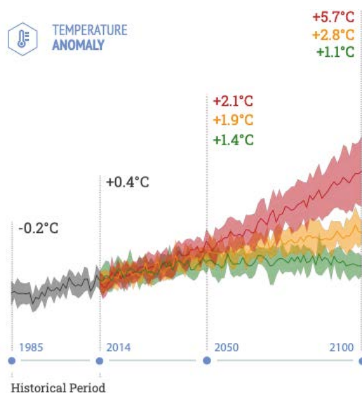
Figure 5: Temperature Projections
